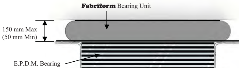
Vertical Bearing Detail
