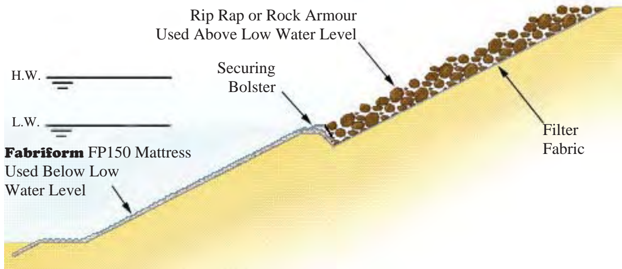
Typical Section
