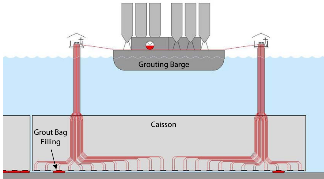
Automated Foundation Grouting
