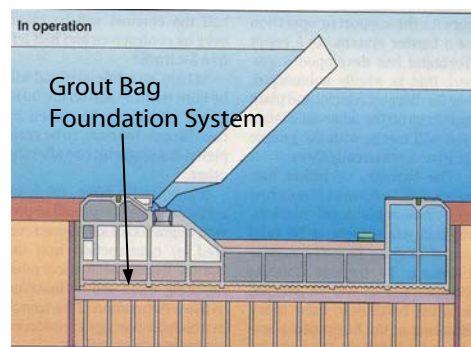
Typical Section
