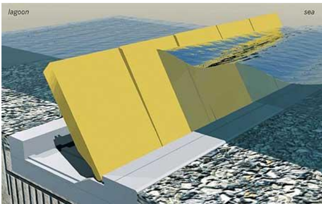
Flap Gates
