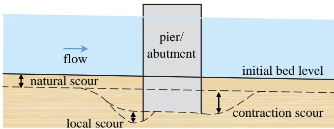
Figure 3. Bridge Scour (CIRIA 2015)
