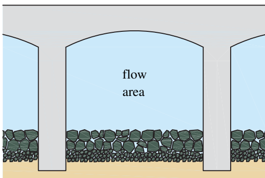
Figure 1. Rock protection
