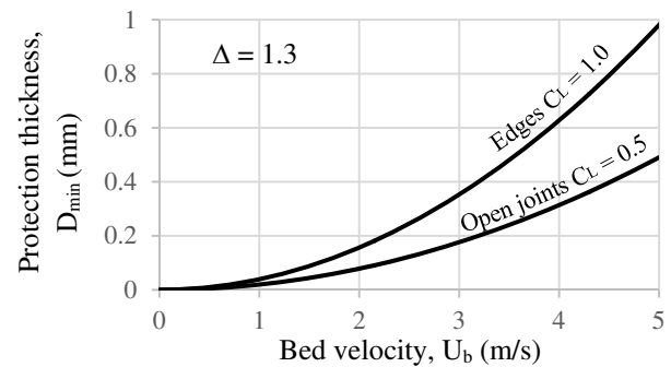
Figure 4. Protection thickness (Raes)
