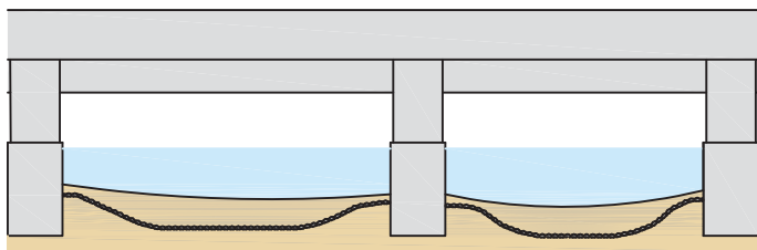
Figure 15. Typical section
