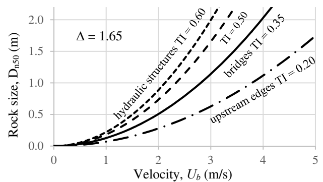
Figure 9. Rock sizes
