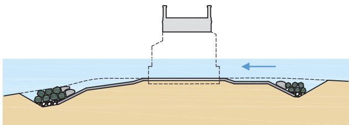
Figure 16. Typical section
