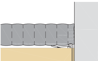
Figure 13. Wall seal
