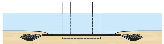
Figure 14. Concrete mattress and rock edge combination.
