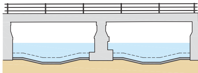
Figure 17. Typical section
