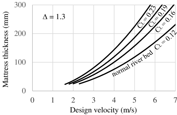
Figure 5. Concrete thickness for turbulent flow at bridges
